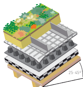
Composition Nophadrain Extensive Green Roof System – steep pitched roof
