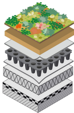
Composition Nophadrain Extensive Green Roof System - inverted roof construction with ND X20 Drainage System
